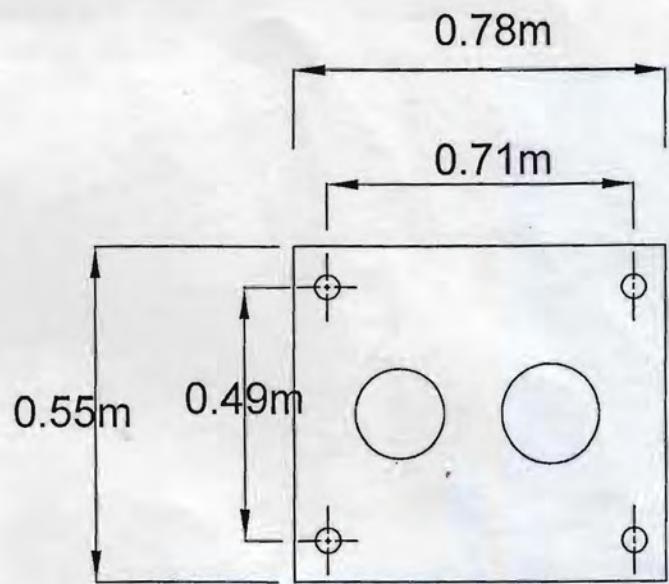
View A-A Base plate
