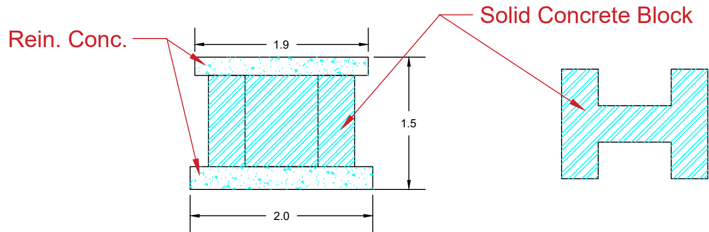
Water Tanks Bases (M-1)
