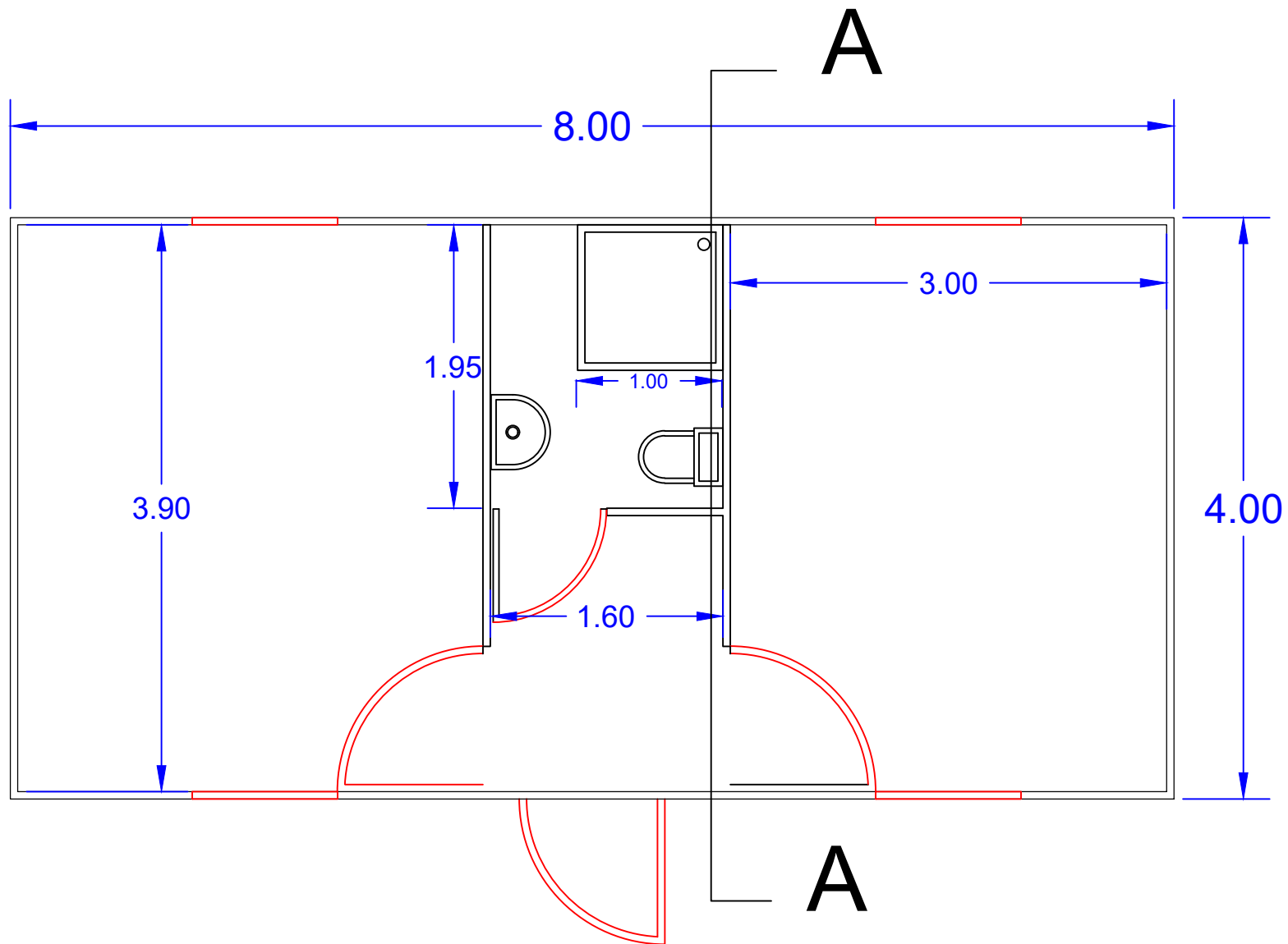
Detail (P-1) - Caravan Plan
