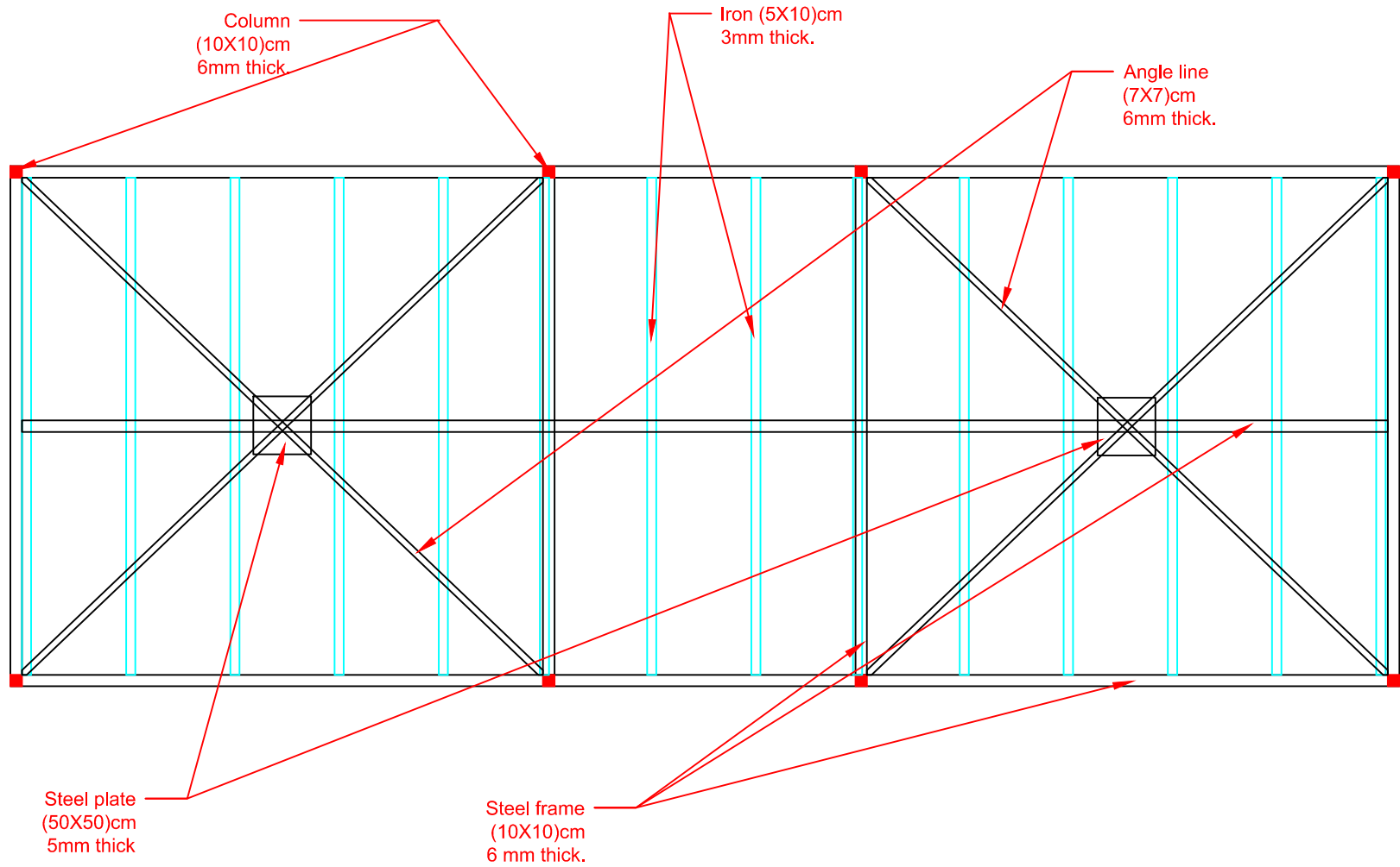
Fig (E - 3) Roof Structure
