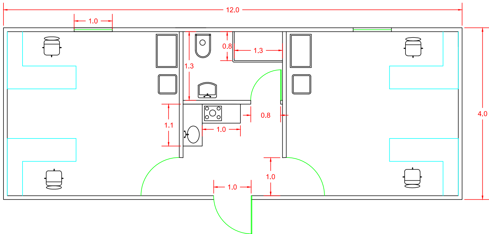
Fig (E - 6) Caravan Items details
