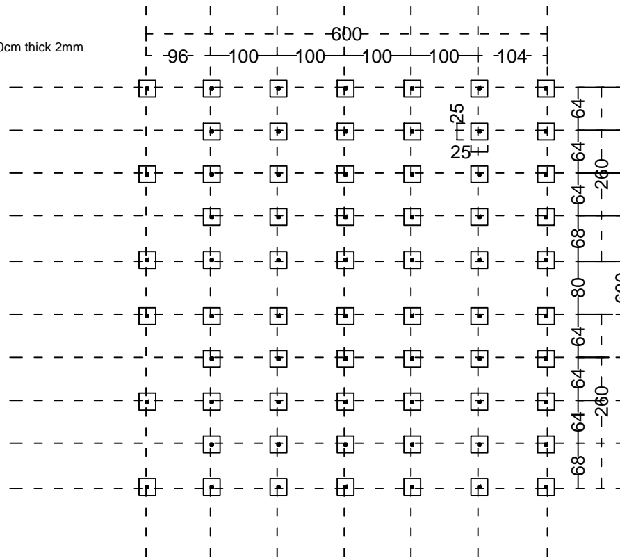
bases for metal poles
