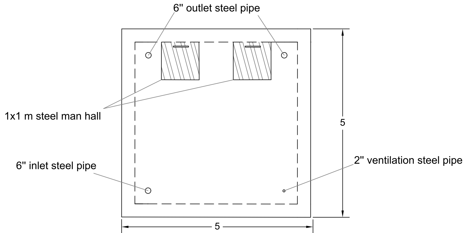
- Top View -
