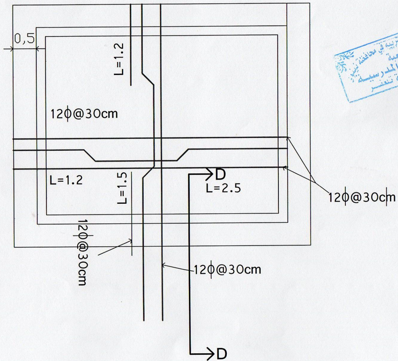
reinforcement plan
