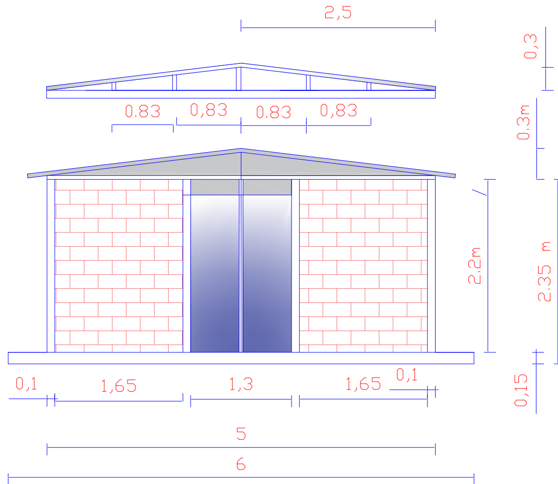
front plan of tents
