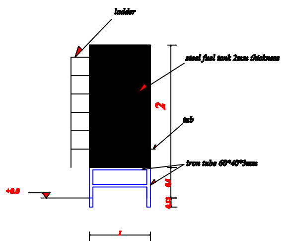
Front view of fuel tank
