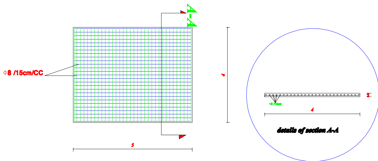
top plan of reinforcement in the base for generator room
