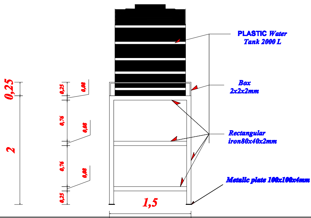
Front view of base tank
