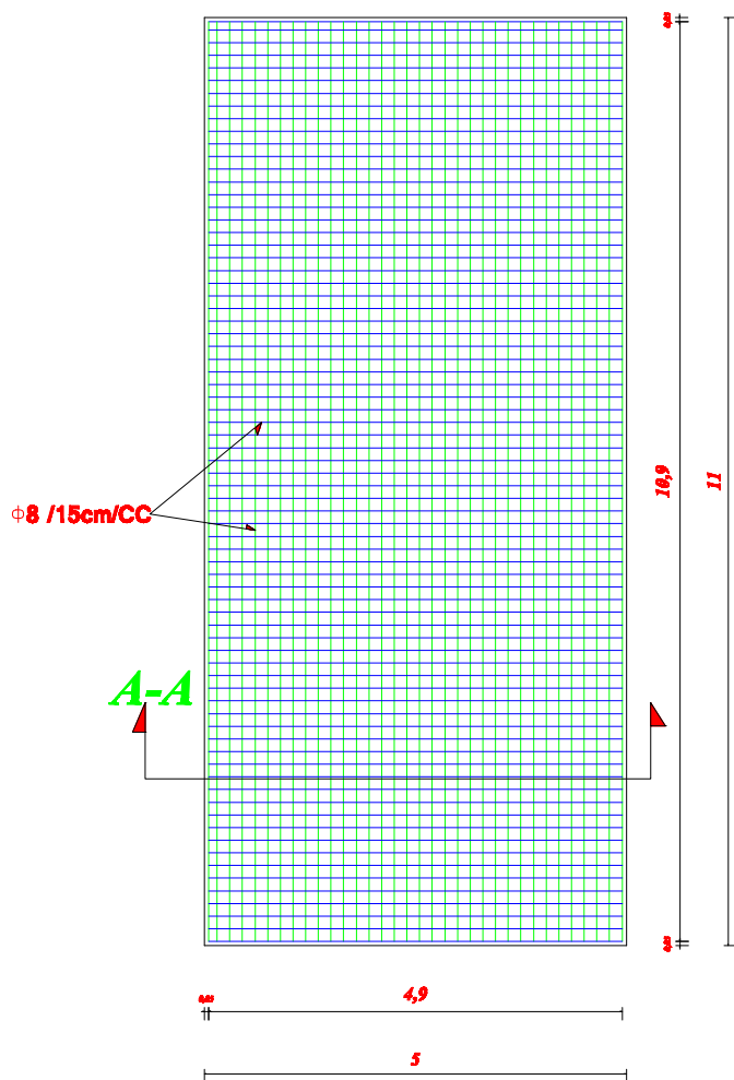
top plan of reinforcement in the base
