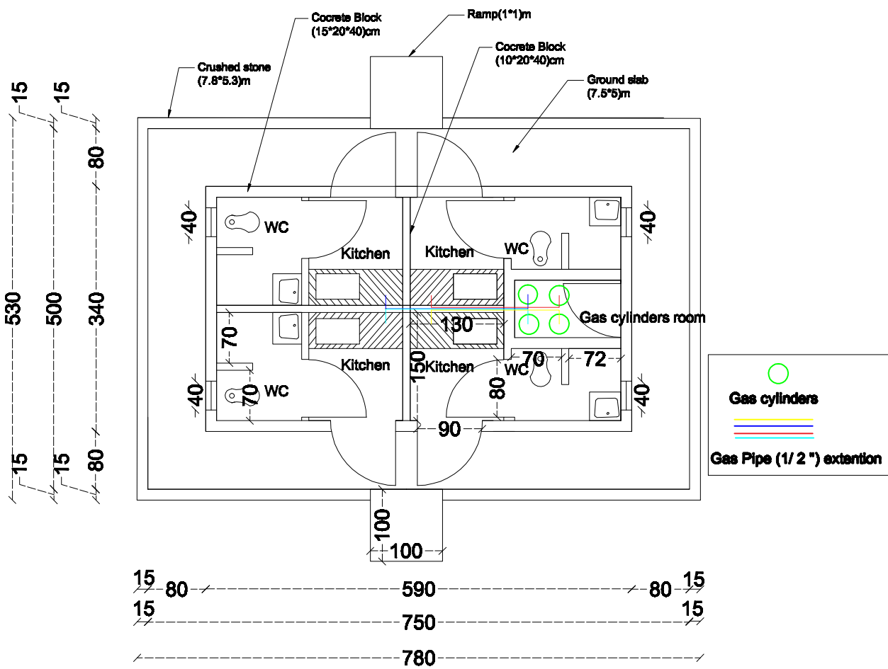
Facility Compound - Gas pipe extensions
