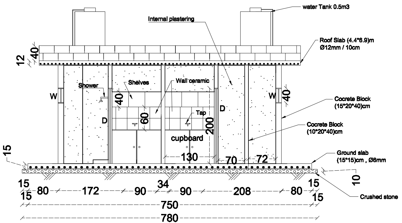
Facility Compound - Section A-A
