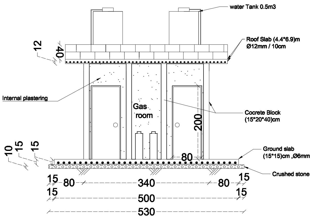
Facility Compound - Section B-B
