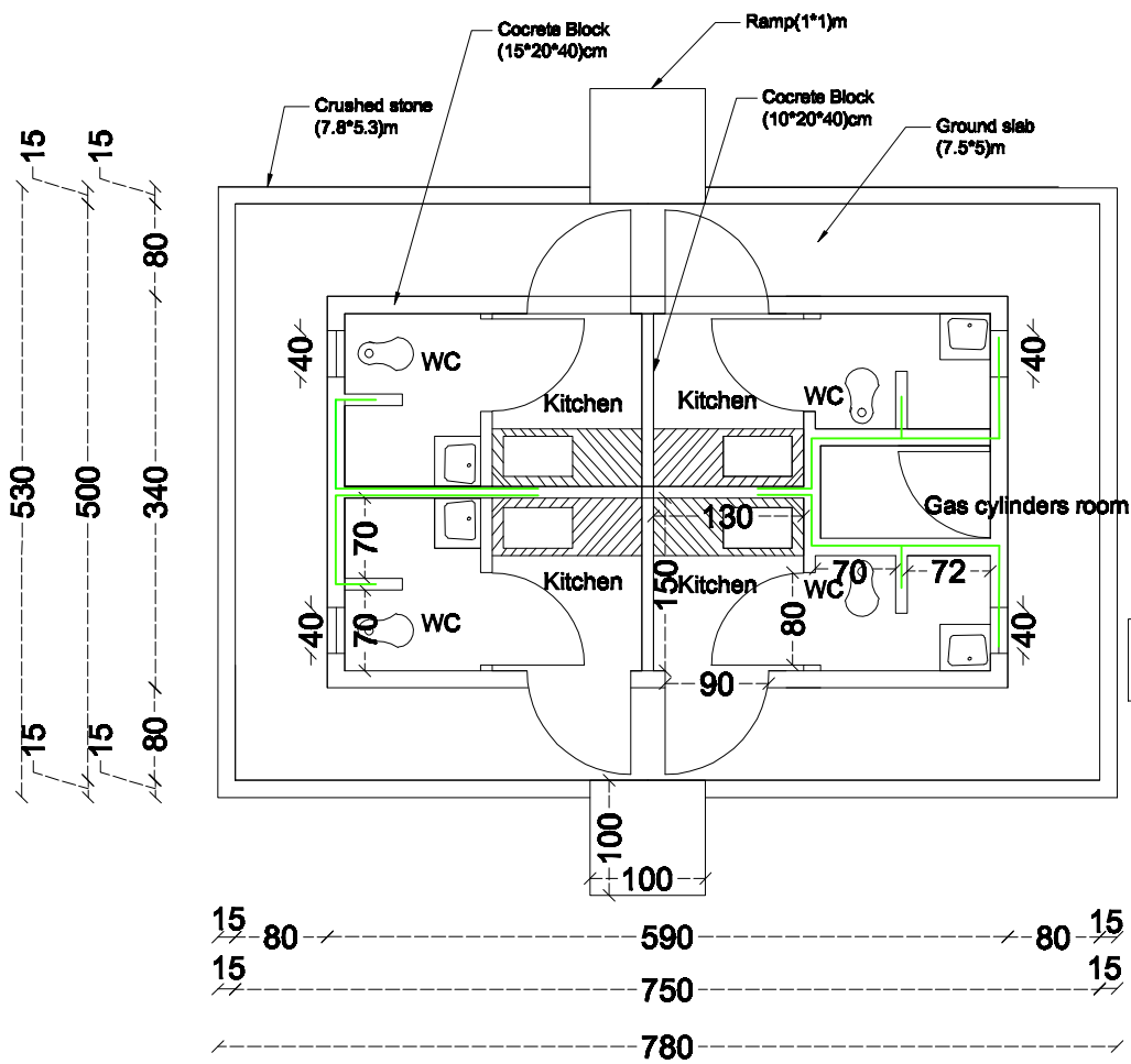
Facility Compound - Water pipe extentionts
