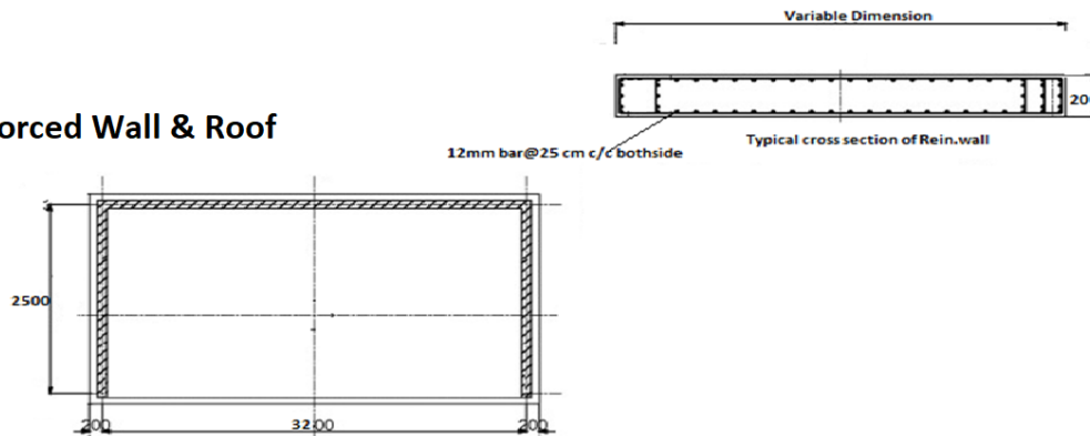
RC Wall
