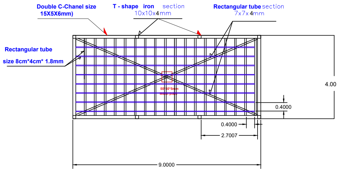
Caravan Base Section
