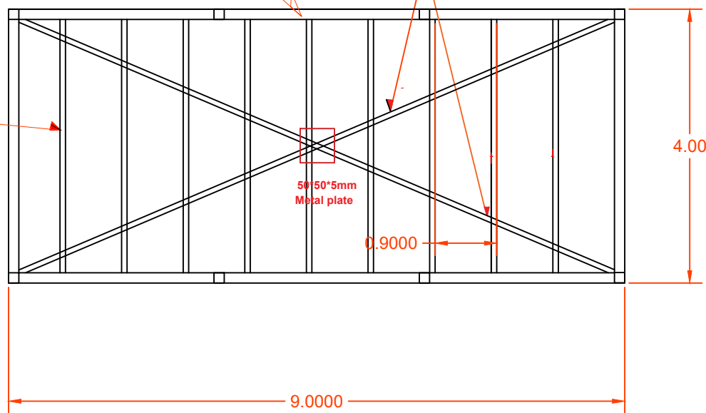
Caravan Roof section
