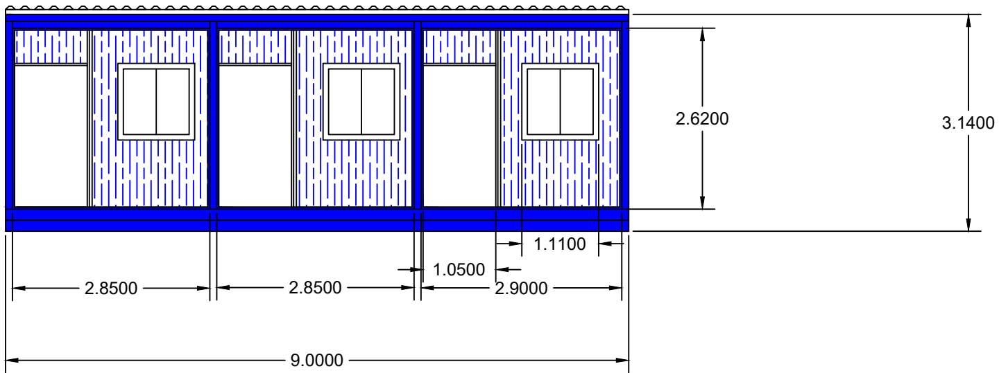
Front Plan
