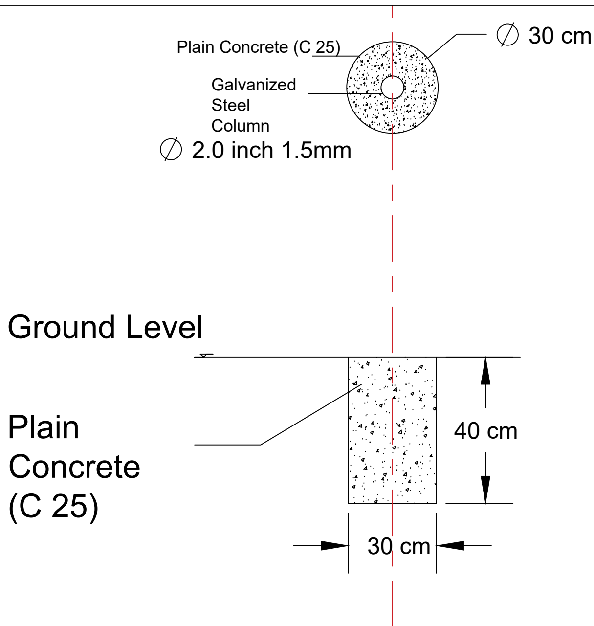
Drawing No. 5 : Concrete bases drawing details
