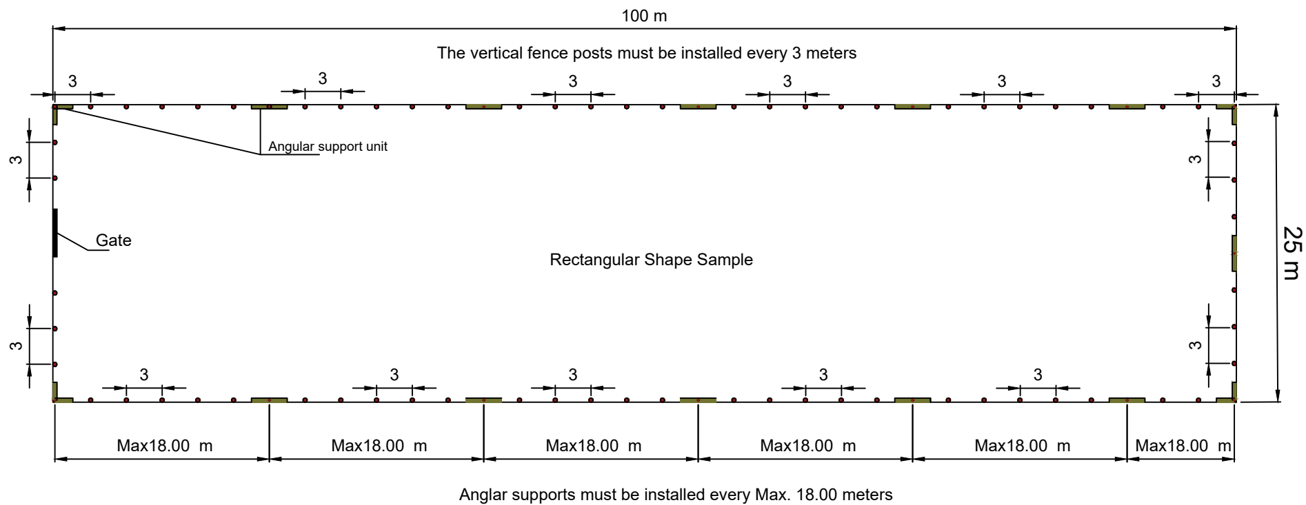
Drawing No. 7 : Rectangular Shape Sample
