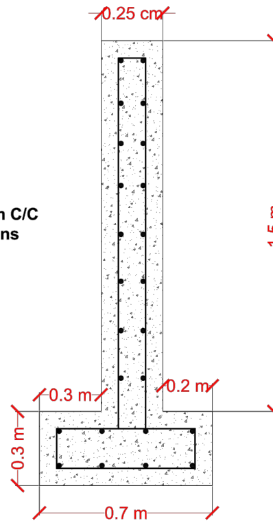
Retaining Wall Cross Section
