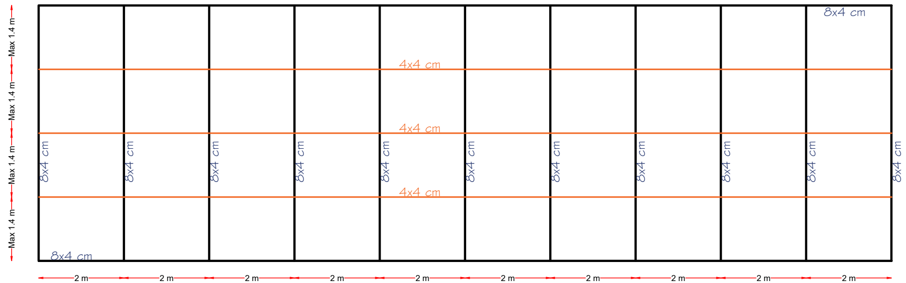
Ceiling Layout
