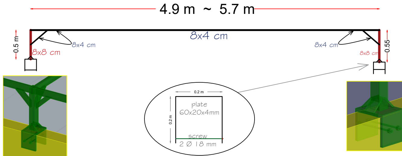
Internal Base Beam Layout
