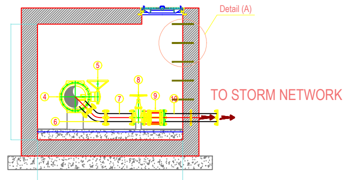
SECTION (C-C)
