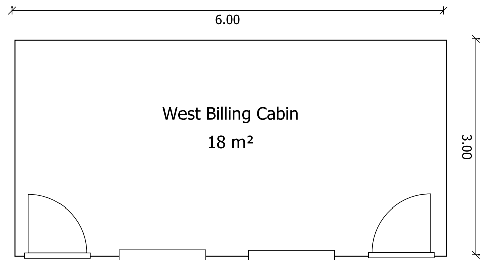
Cabin No.3 West Mosul cabin 6 x 3 x 2.8
