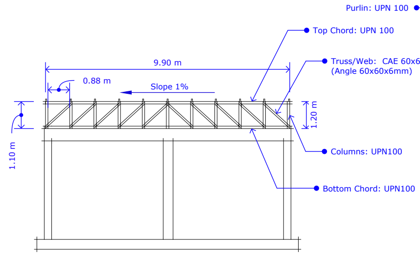
15 A STEEL DESIGN SIDE SCALE 1:150
