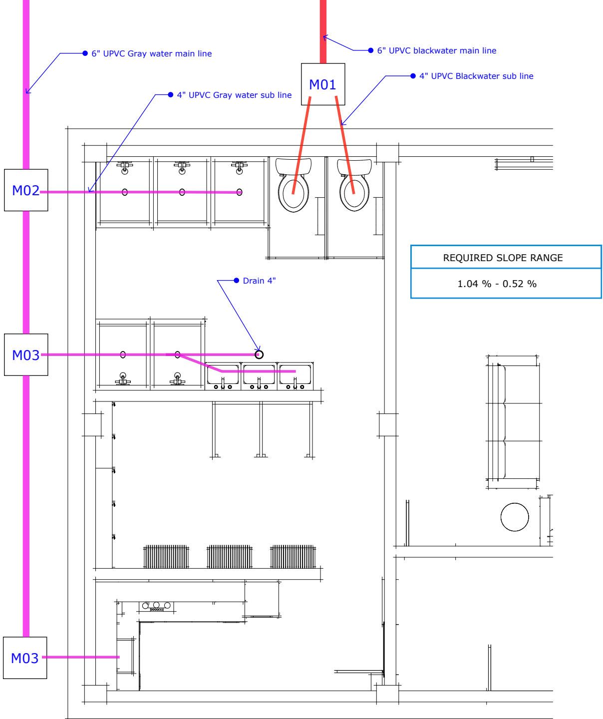
02 M WASTE WATER SYSTM SCALE 1:67
