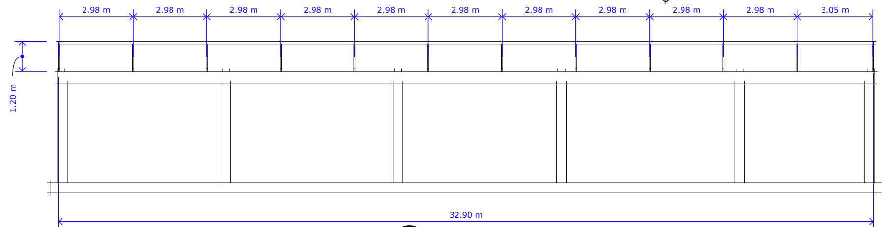
14 A STEEL DESIGN FRONT SCALE 1:150
