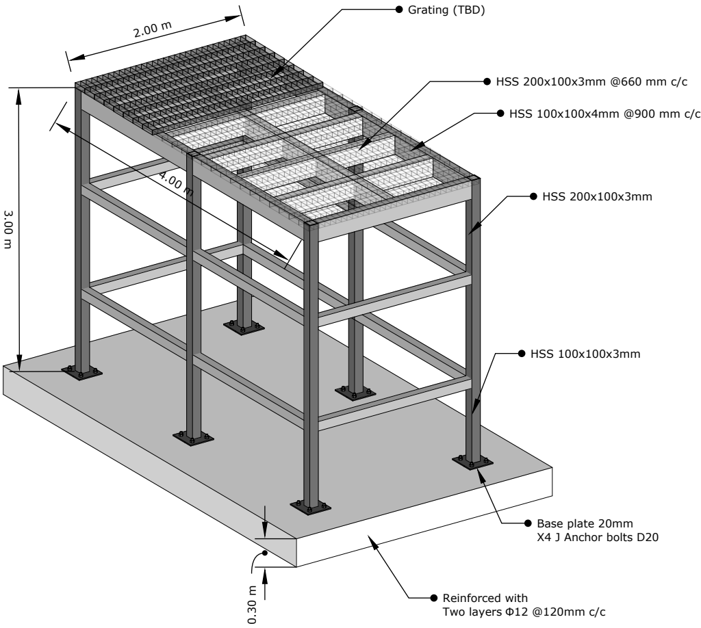
03 Structural details SCALE 1:50
