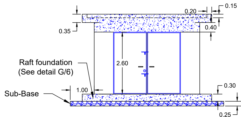
Front view
