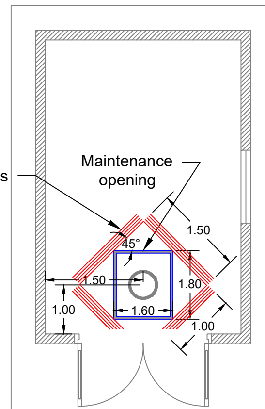
Top View
