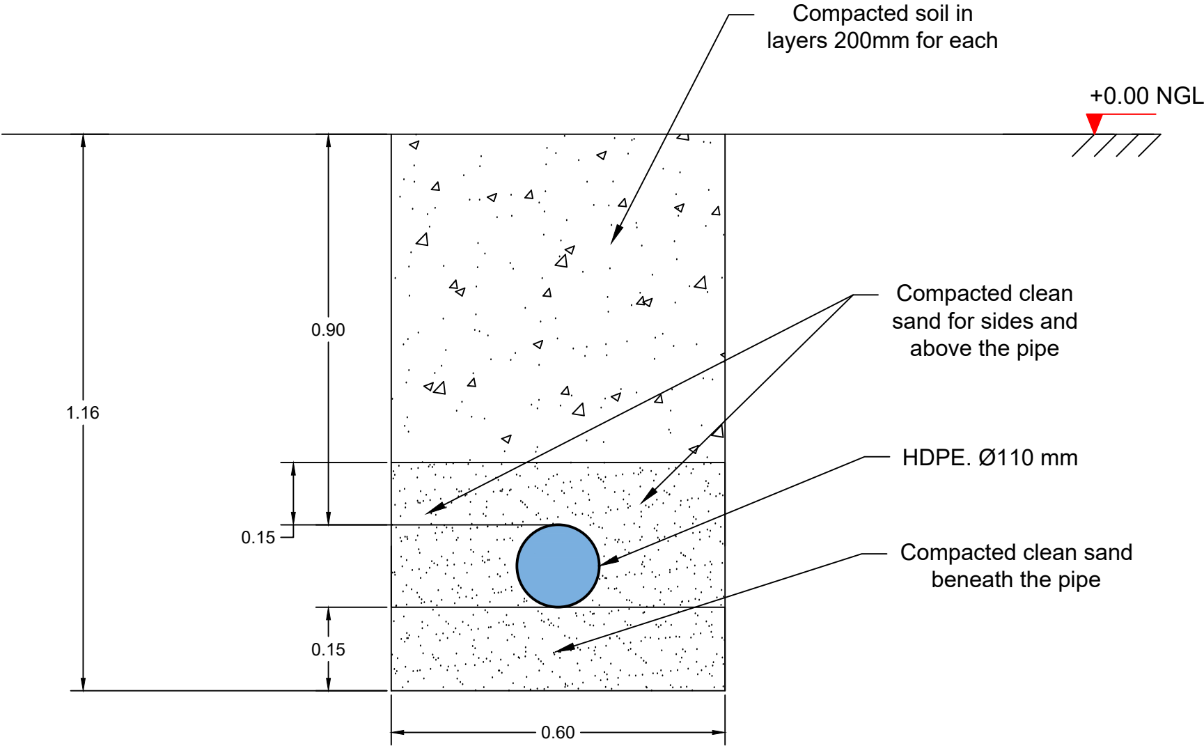
Pipe Trench Cross Section
