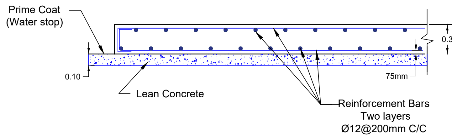
Detail G Raft foundation (Room)
