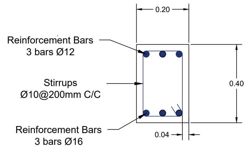
Detail Y Concrete Beam
