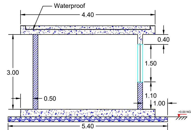
Section(A-A) Room Cross Section
