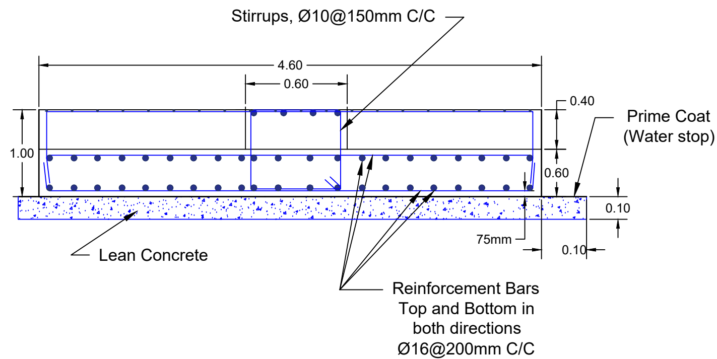
Section(B-B) Details H
