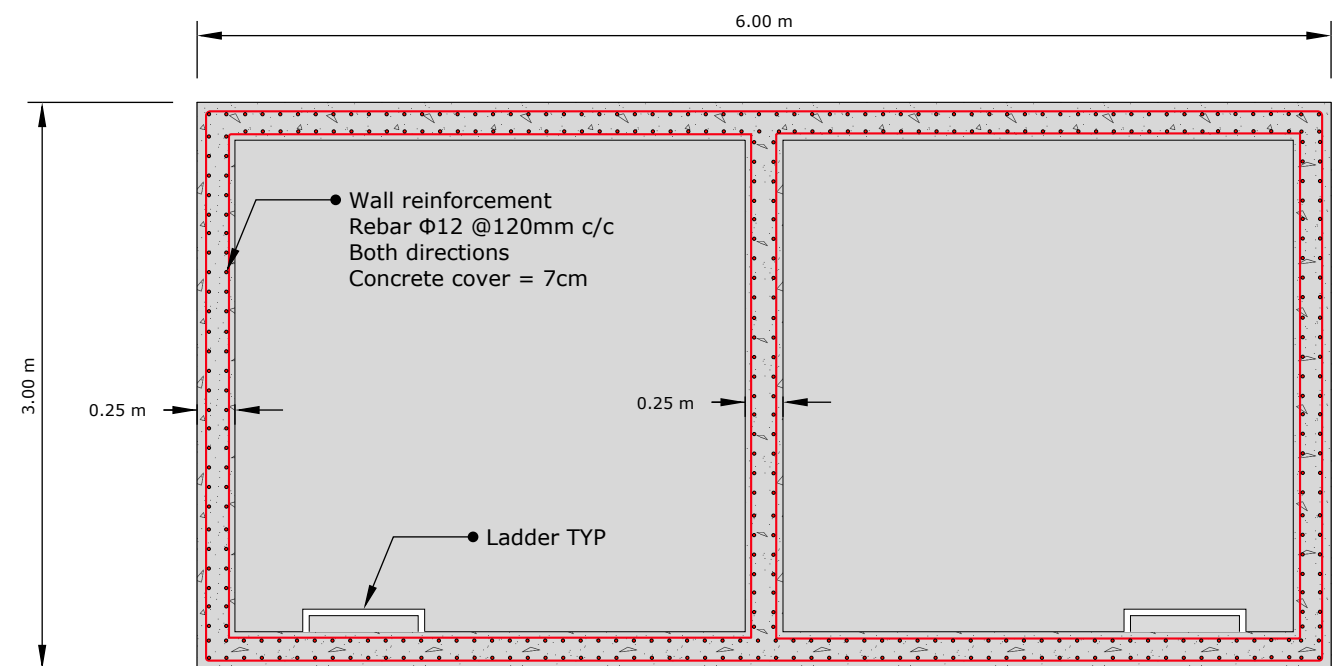
05 SECTION 5-5 S SCALE 1:40
