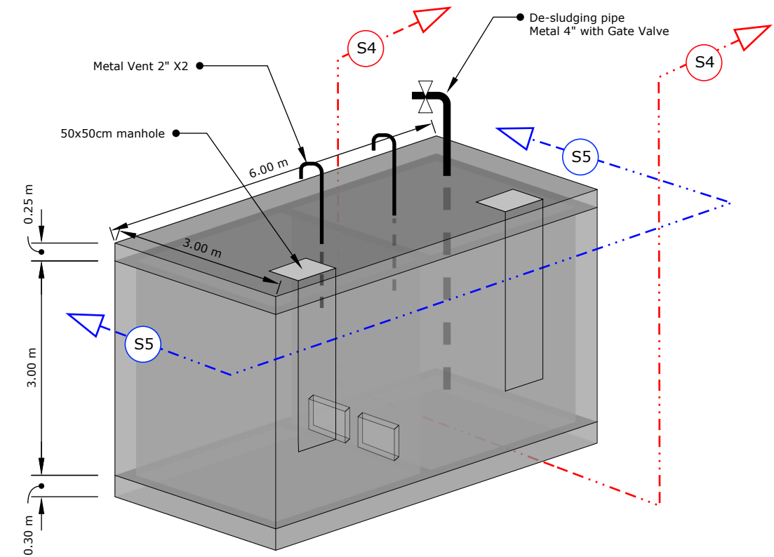
07 SEPTIC TANK DETAILS M SCALE 1:70
