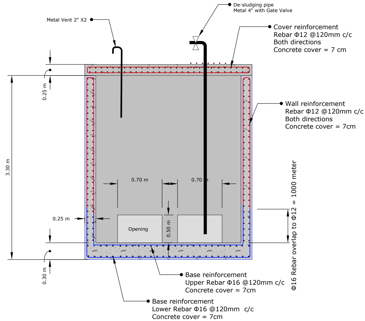
04 SECTION 4-4 S SCALE 1:40
