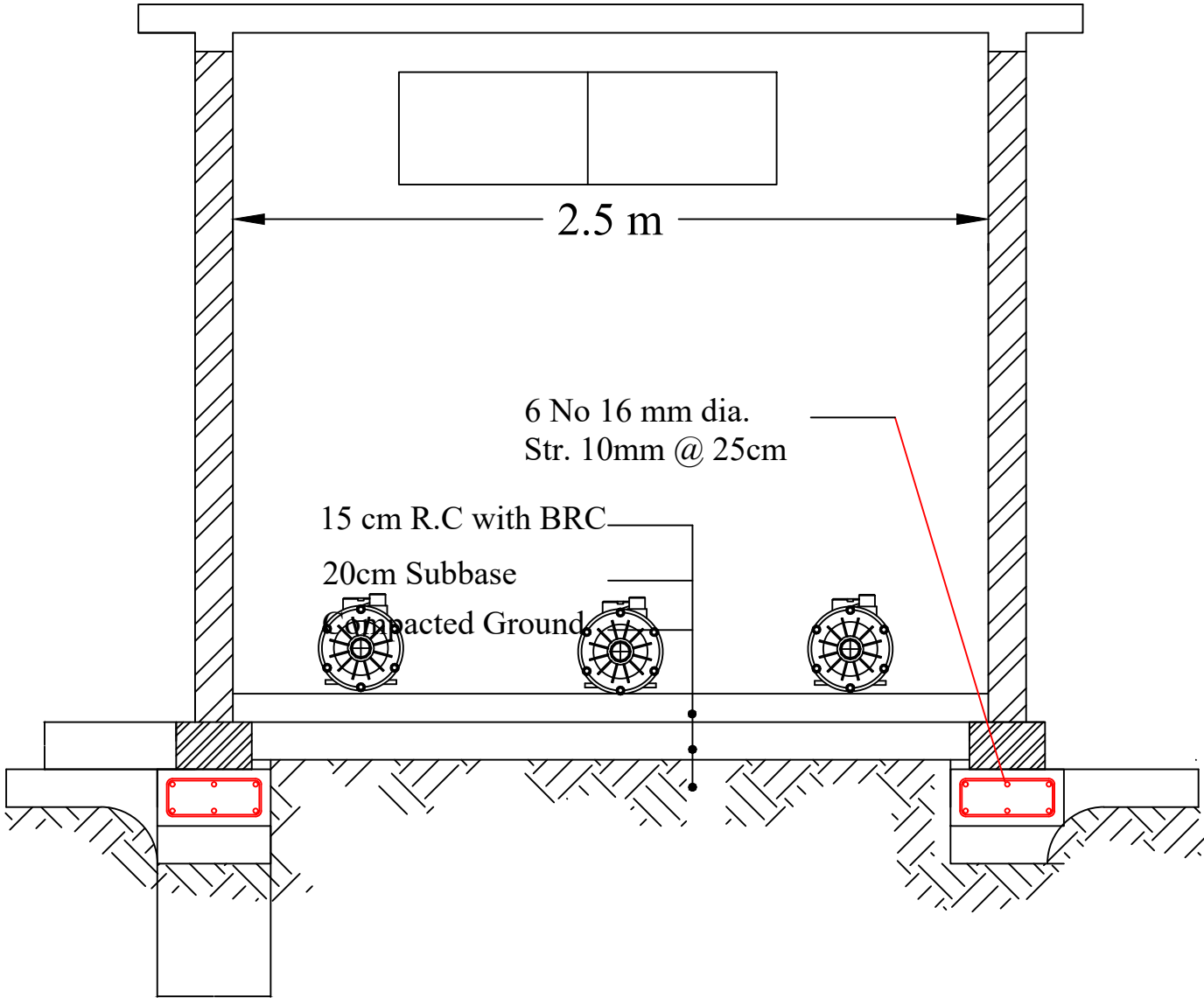
Section B-B
