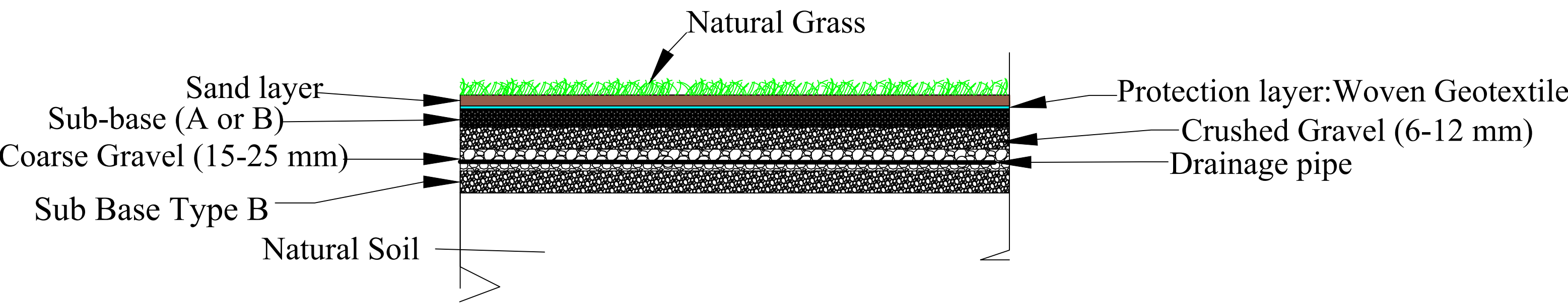
Section of backfilling
