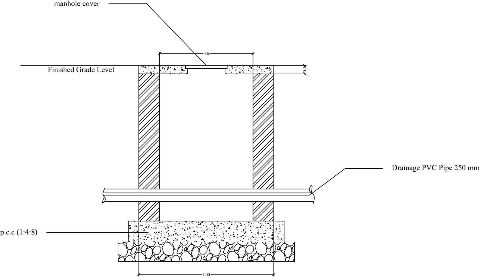
Front view Manhole
