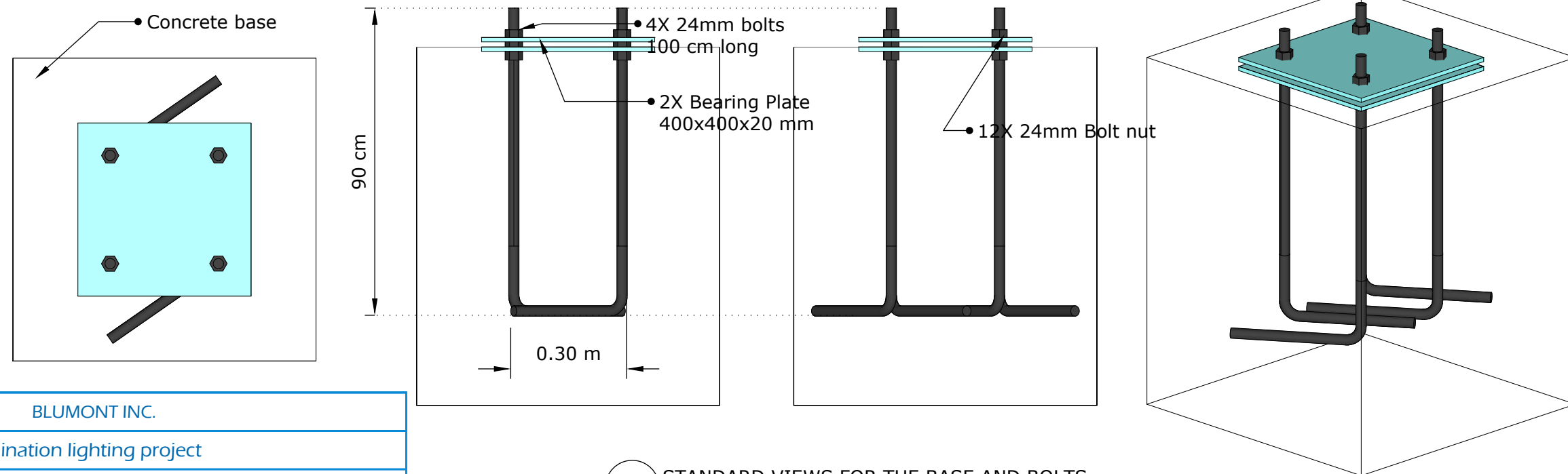
A4 STANDARD VIEWS FOR THE BASE AND BOLTS NOT TO SCALE
