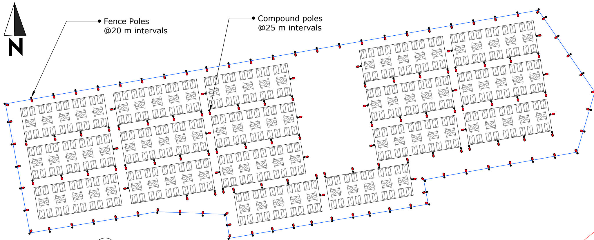
A1 SITE PLAN NOT TO SCALE
