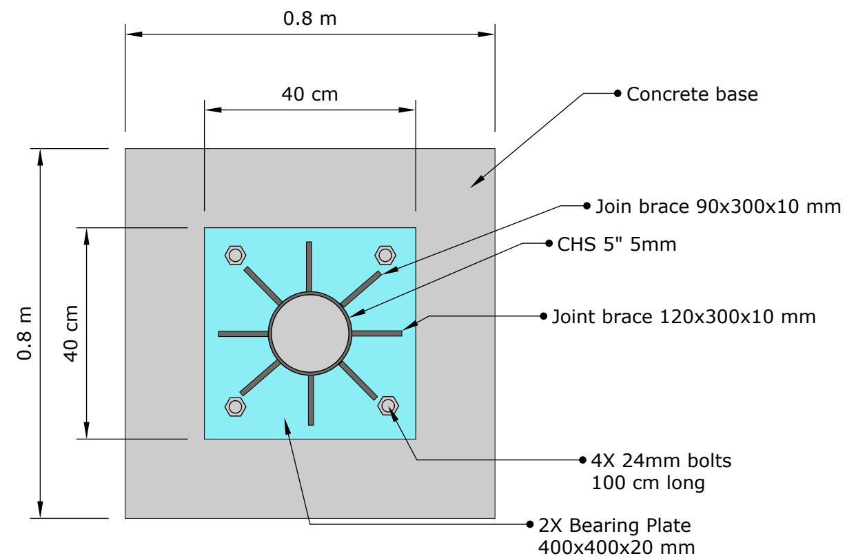
A3 CONCRETE BASE AND CONNECTION DETAILS NOT TO SCALE
