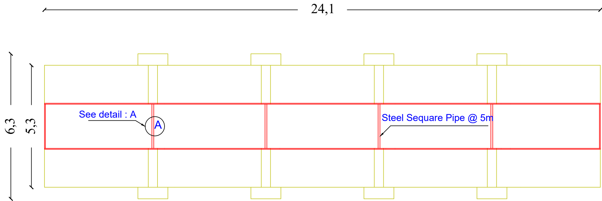
hand rail plan
