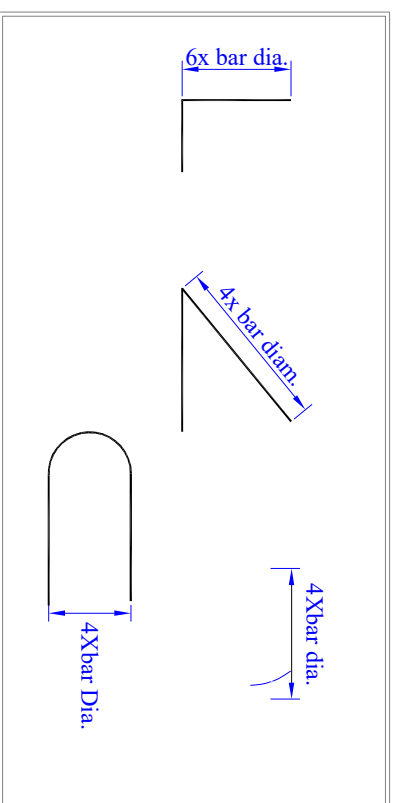
Detail of Hook of Bars
