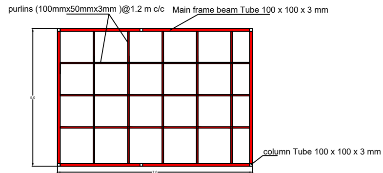
Steel Structure details of ceiling
