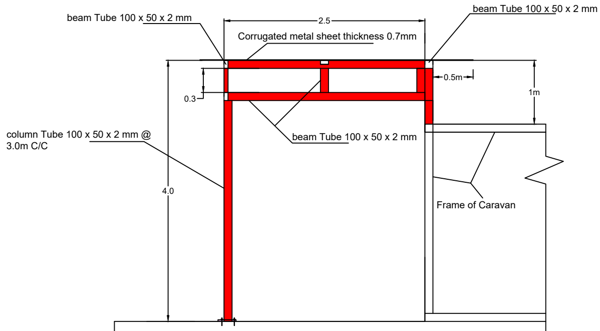
Details of Sun Shed connected with Classrooms
