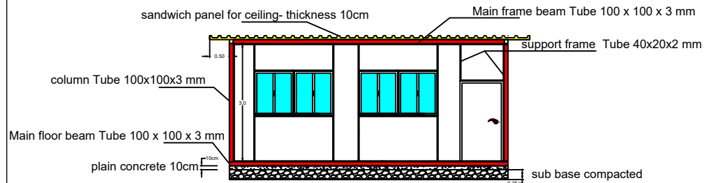
Steel Structure and Sandwich Panel ( front view)
