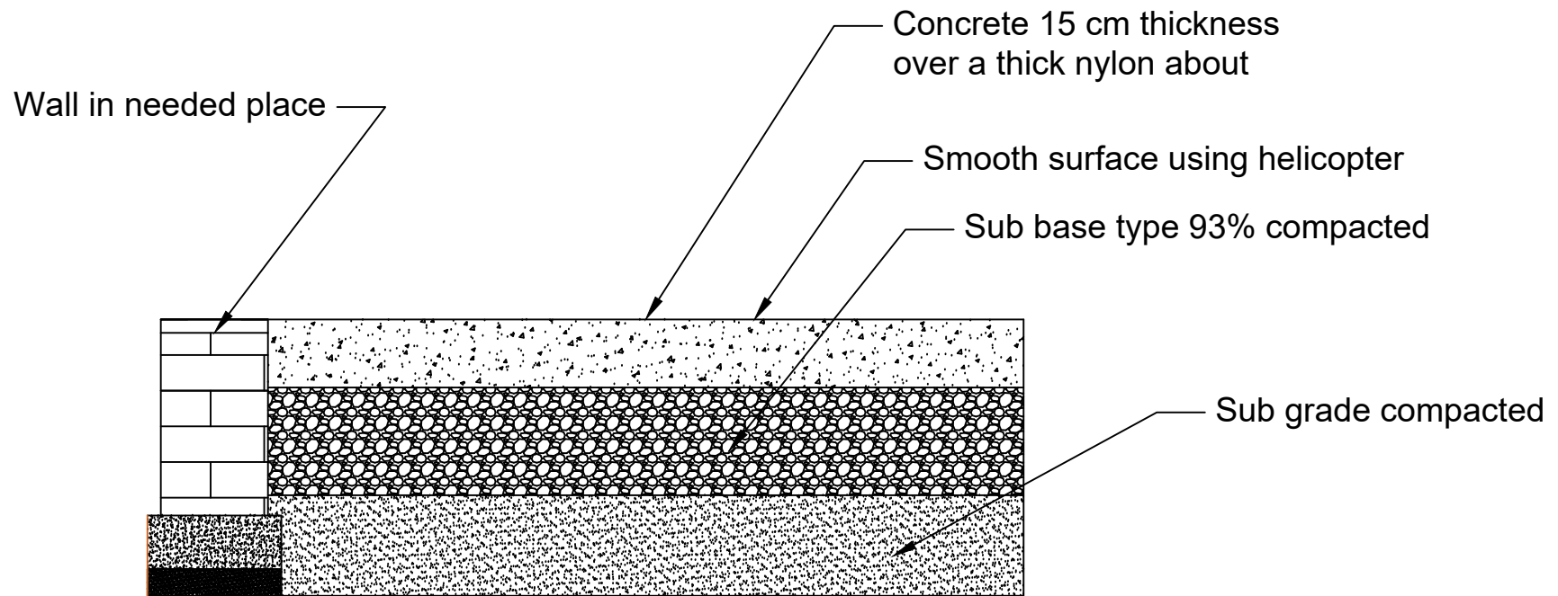
Concrete section
