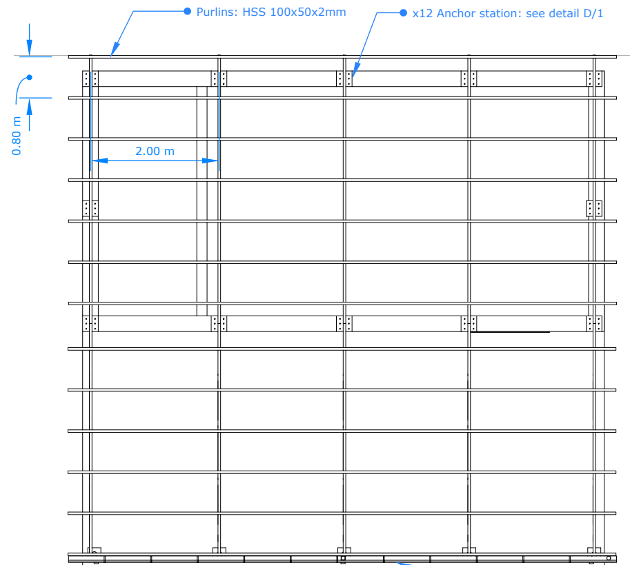
10 CCC ROOF STEEL PLAN A SCALE: 1:100
