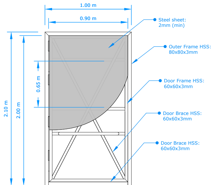
03 B CASE MANAGEMENT DOOR SCALE 1:30
