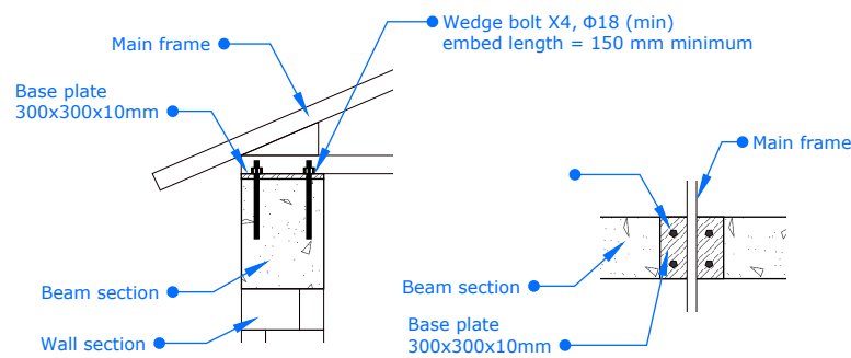
01 ANCHOR STATION D NOT TO SCALE
