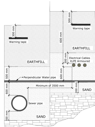
02 INFRASTRUCTURAL SPACEING E NOT TO SCALE
