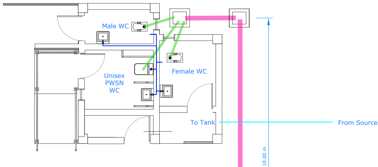
30 PLUMBING PLAN A SCALE 1:70
