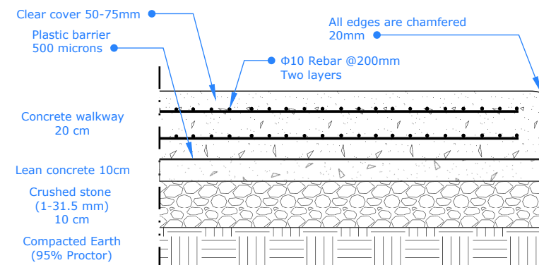
27 A WALKWAY DETAILS NOT TO SCALE
