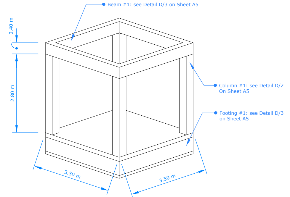
37 SKELETON ISO A SCALE 1:75
