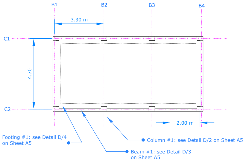
09 CC COMPOUND CONCRETE PLAN A SCALE: 1:150
