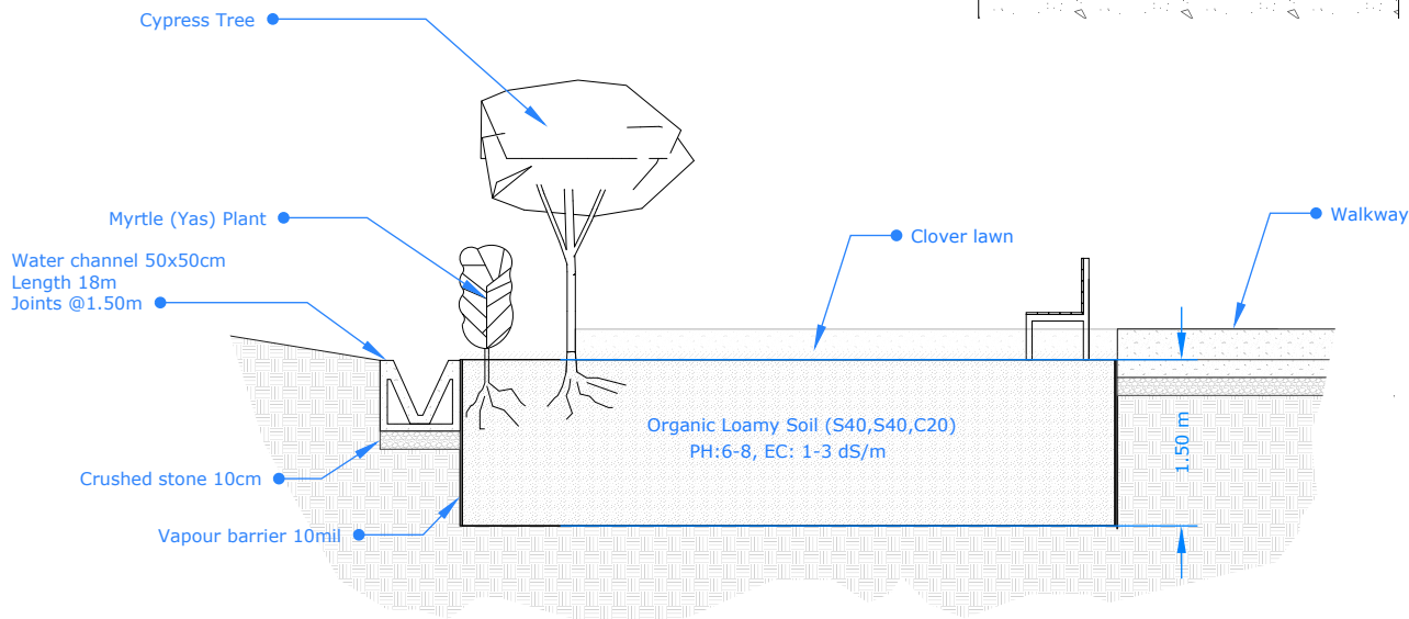
04 GARDEN SECTION S SCALE 1:110
