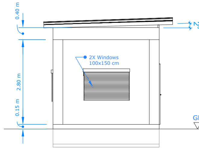
32 SIDE VIEW A SCALE 1:75
