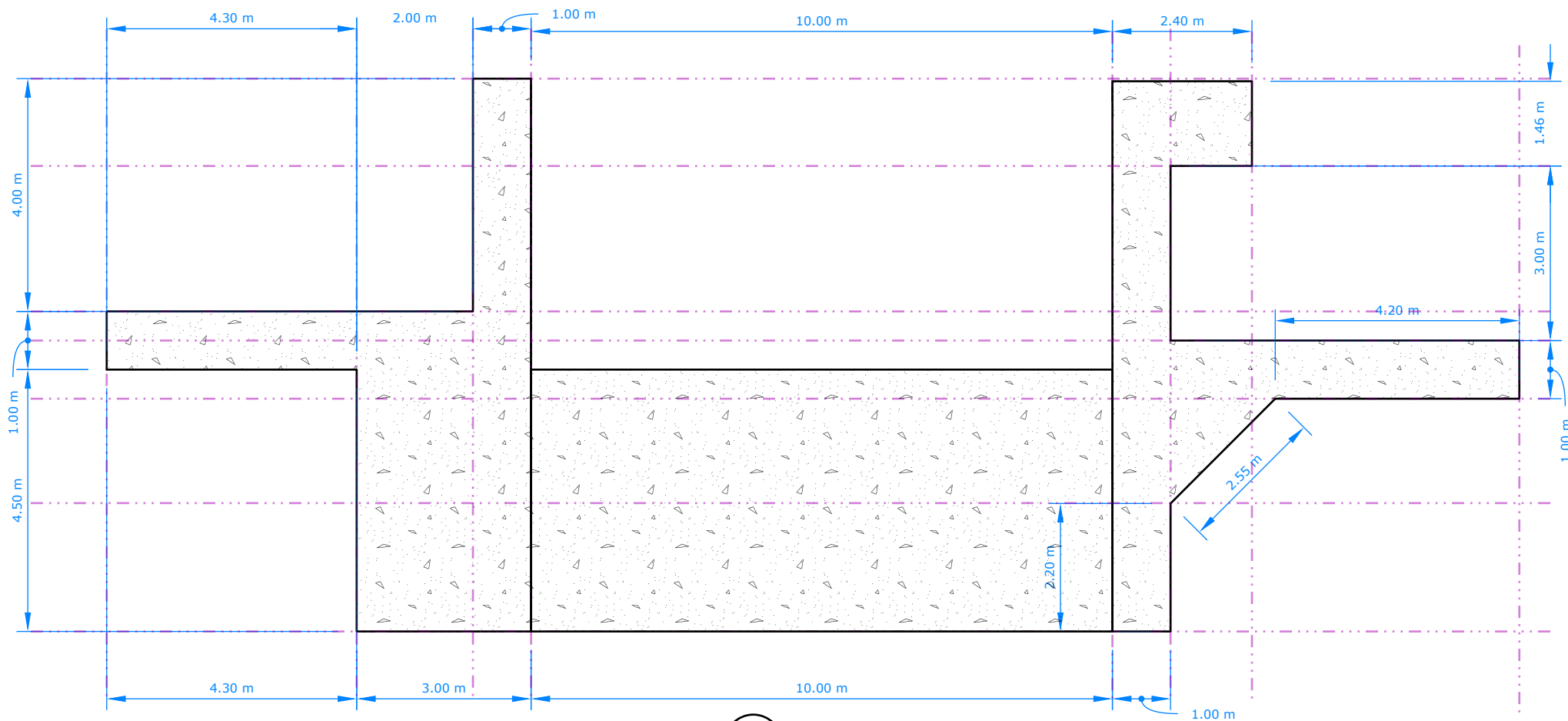
28 A WALKWAY PLAN SCALE 1:100
