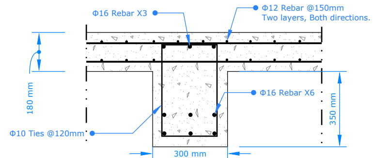
01 E LAATRINE SLAB NOT TO SCALE
