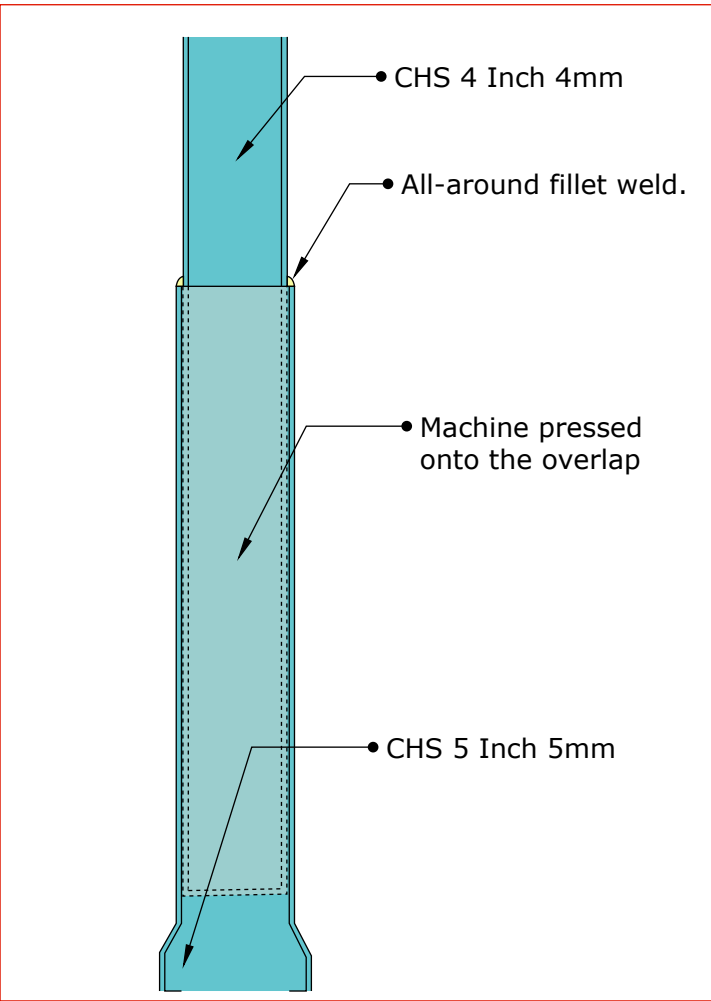
03 A PROTECTION AGAINST CLIMBING NOT TO SCALE
