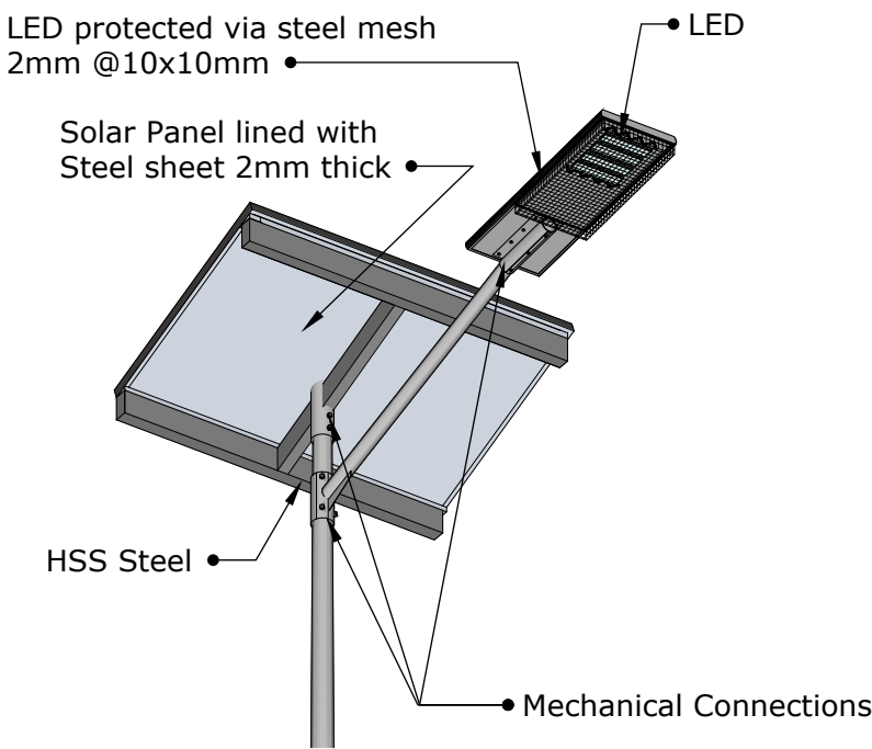
02 A PROTECTION AGAINST PROJECTILES NOT TO SCALE
