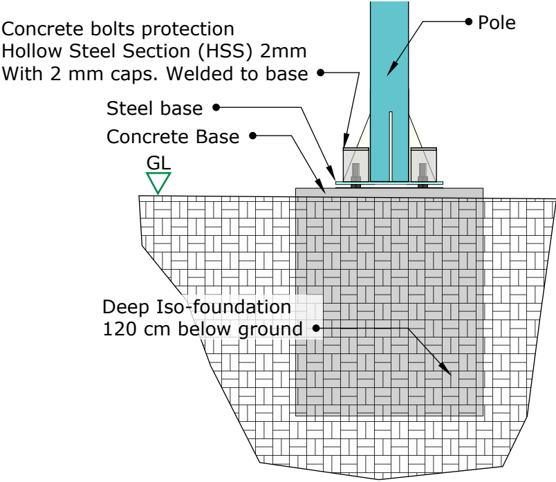
04 A PROTECTION AGAINST OVERTURNING NOT TO SCALE
