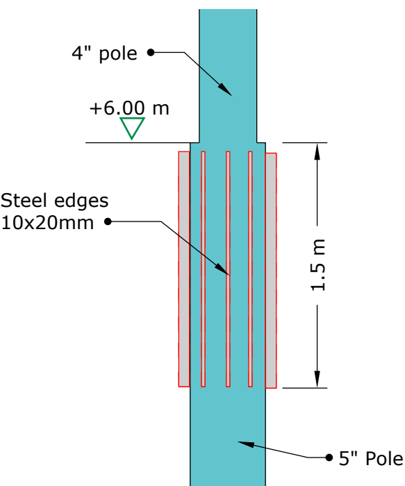
03 A PROTECTION AGAINST CLIMBING NOT TO SCALE
