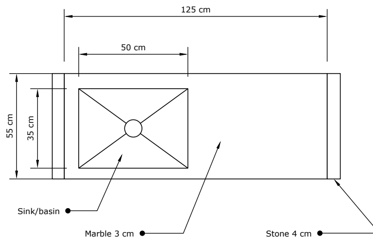
A 22 KITCHEN MARBLE NOT TO SCALE
