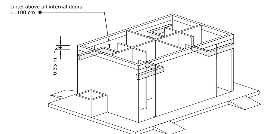
A 09 BEAM DETAILS ISO VIEW SCALE 1:100
