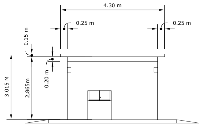
A 10 SLAB DETAILS SIDE VIEW SCALE 1:100
