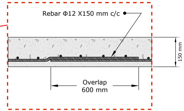
D 03 SLAB DETAILS SIDE VIEW NOT TO SCALE
