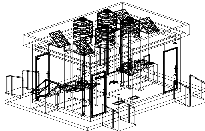
A 13 COMPLETE ITPFQ ISO VIEW SCALE 1:100
