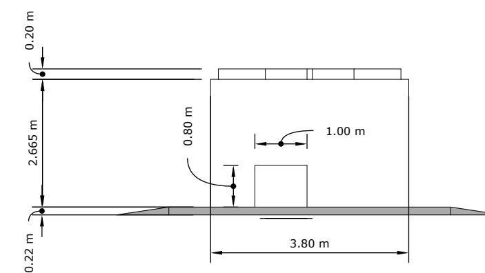
A 03 WALLS STRUCTURE DETAILS SCALE 1:100
