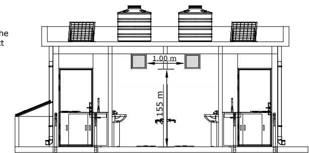
A 14 COMPLETE ITPFQ FRONT VIEW SCALE 1:100
