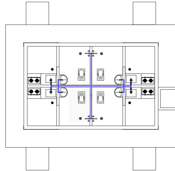
A 16 WATER DISTRIBUTION PLAN SCALE 1:100
