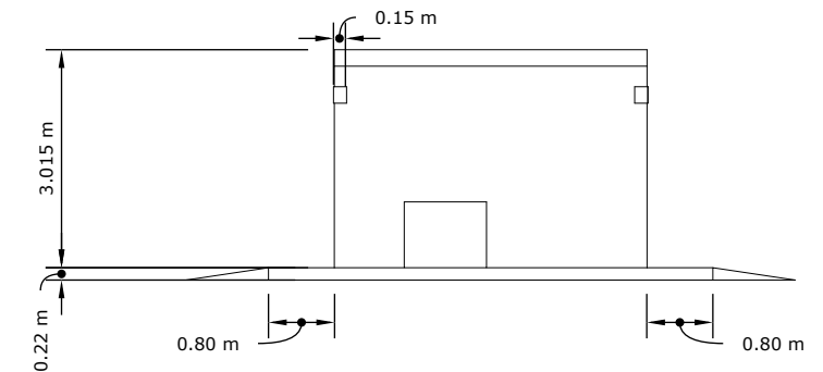
A 08 BEAM DETAILS SIDE VIEW SCALE 1:100
