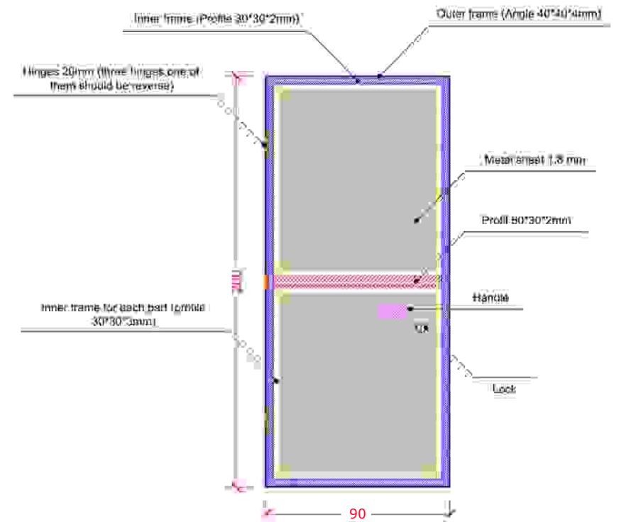
A 21 DOOR DETAILS NOT TO SCALE
