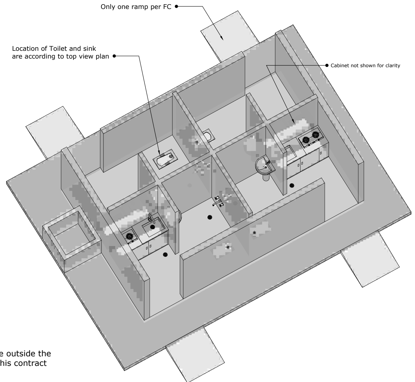
A 05 INTERIOR PLAN (XRAY) ISO SCALE 1:50
