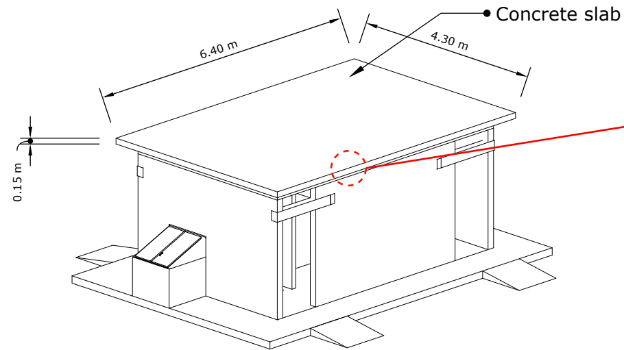
A 11 SLAB DETAILS ISO VIEW SCALE 1:100
