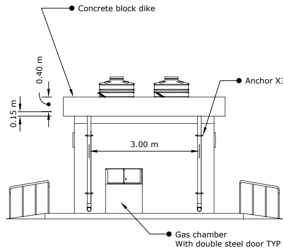
A 12 COMPLETE ITPFQ SIDE VIEW SCALE 1:100
