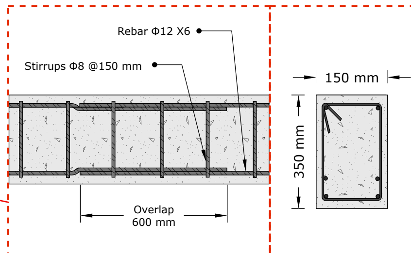
D 01 BEAM #1 DETAILS NOT TO SCALE
