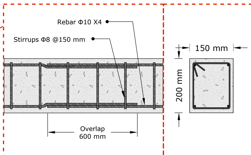
D 02 BEAM #2 DETAILS NOT TO SCALE
