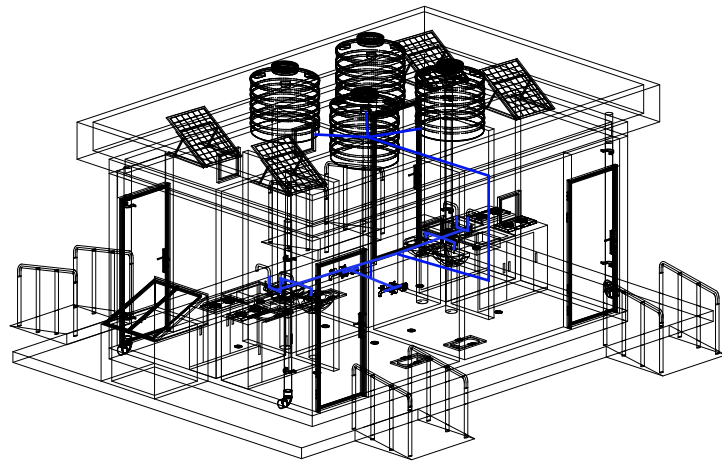
D 05 WATER SUPPLY WIREFRAME SCALE 1:100
